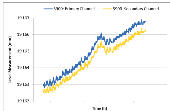
Tracking of dual level measurements from one 2-in-1 radar gauge (NOTE: an offset between measurements has been added for illustrative purposes)
